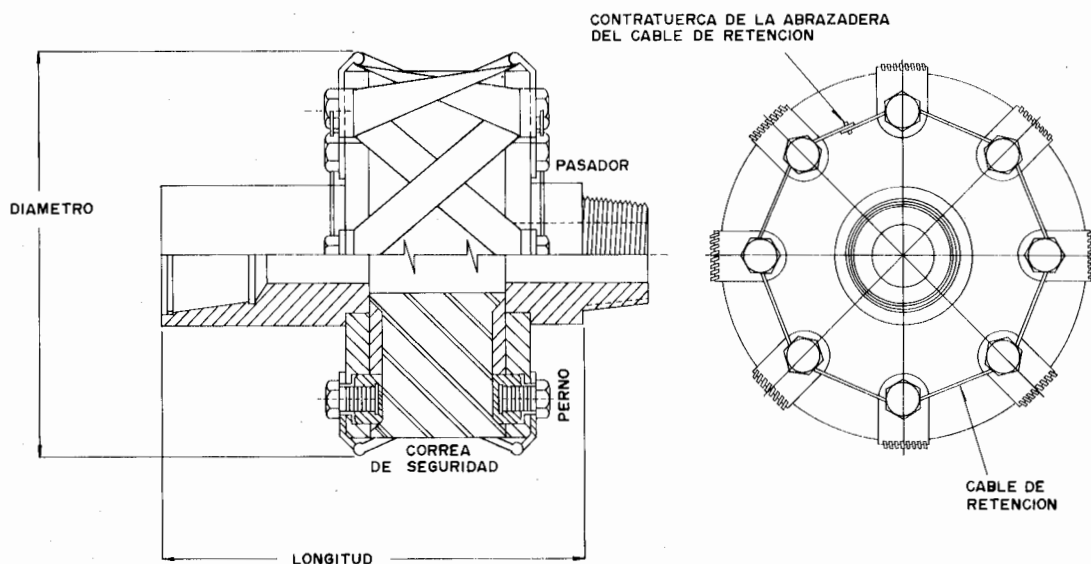
Figura 4.12. Amortiguador vertical (B. J. Hughes Inc.).
